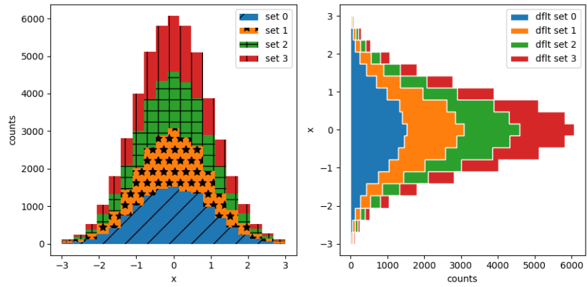
Fig. 7: Filled Step
