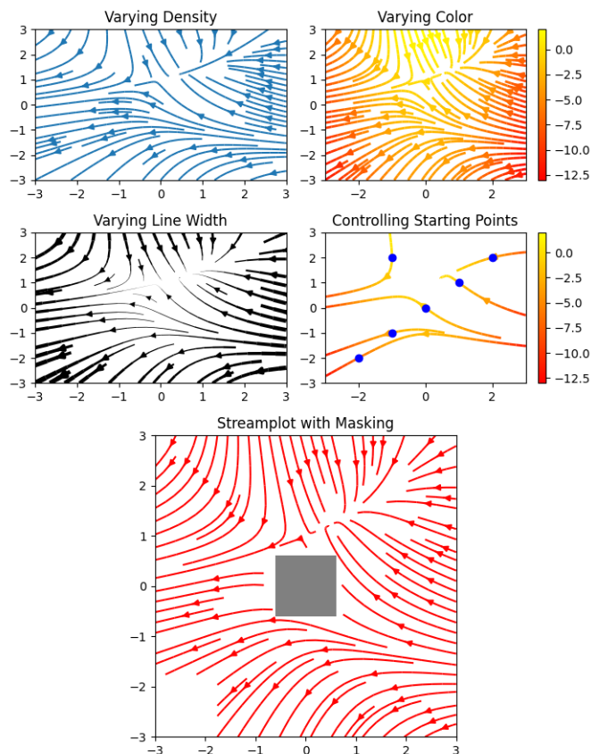
Fig. 18: Plot Streamplot
