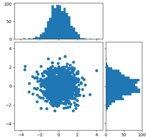
Fig. 52: Scatter Hist
