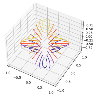
Fig. 11: Tricontour3d
