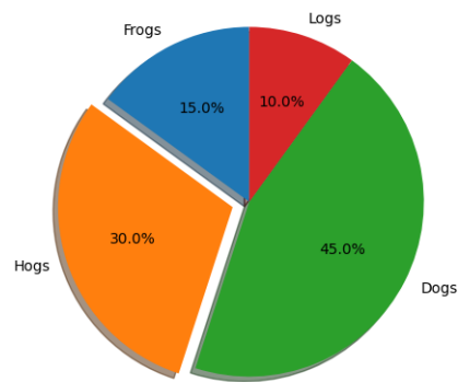
Fig. 11: Pie Features
