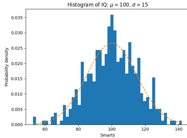
Fig. 5: Histogram Features
