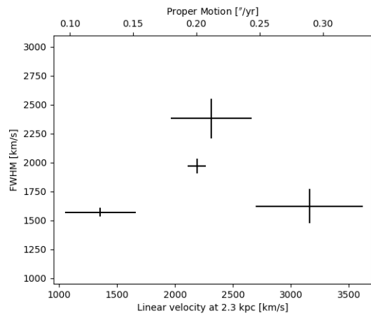
Fig. 55: Parasite Simple2
