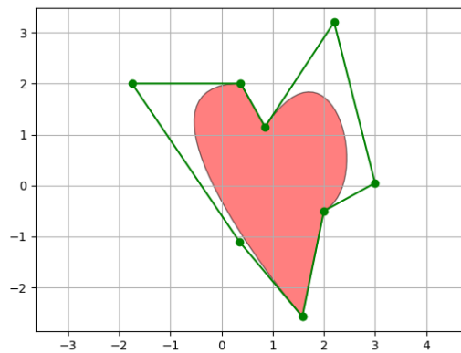
Fig. 6: Path Patch
