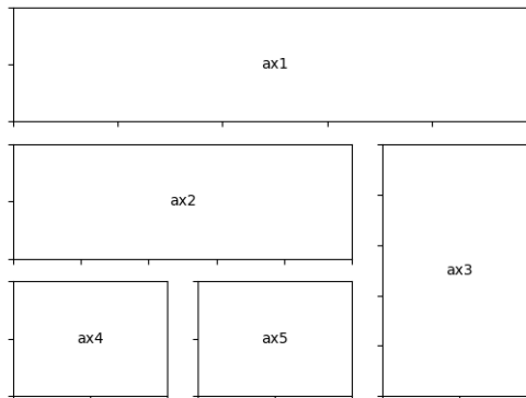
Fig. 25: Demo Gridspec01
