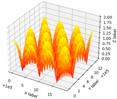
Fig. 23: Offset
