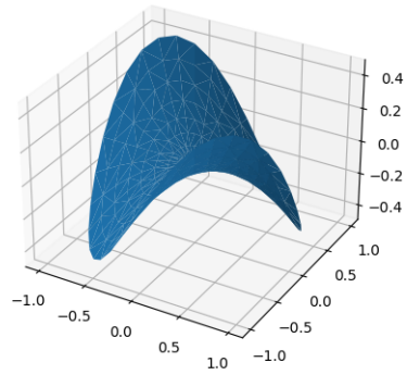
Fig. 16: Trisurf3d
