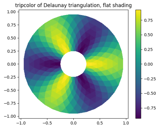
Fig. 19: Tripcolor Demo
