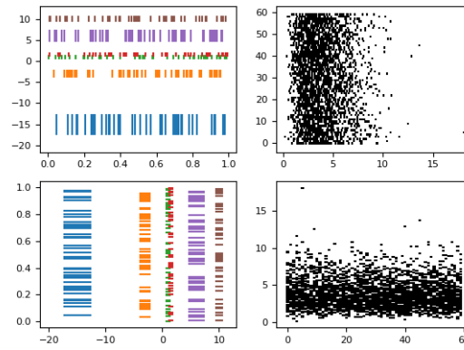
Fig. 12: Eventplot Demo
